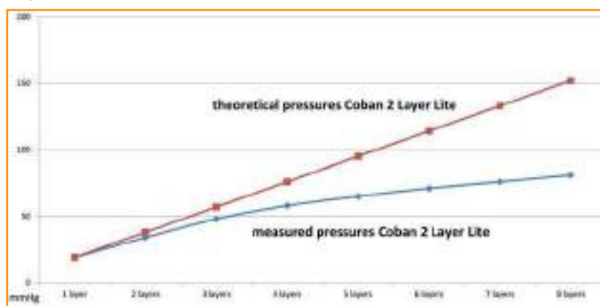
Figure 2: Theoretical and measured pressure values of Coban® 2 Layer Lite
