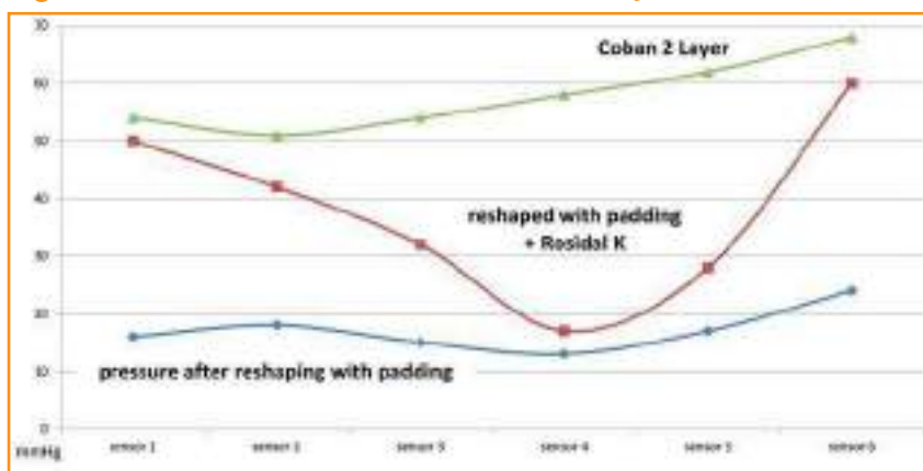
Figure 8: Pressure profile of the materials under investigation on the leg with the narrowed area around the ankle joint
